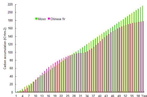
Figure 2 above: Predicted accumulation of carbon stock over a 60 year time period with regular harvesting practices (t C/ha)
